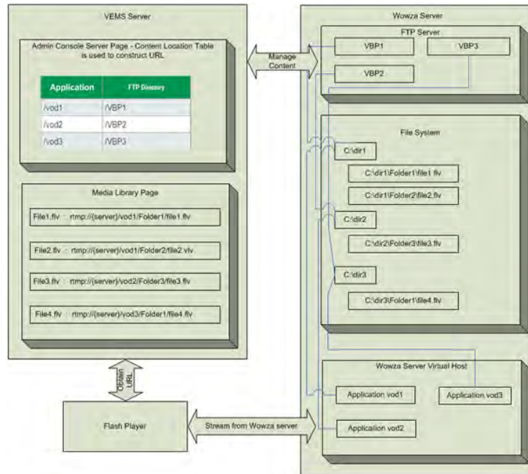
Figure 6. Wowza VOD Server File Structure
