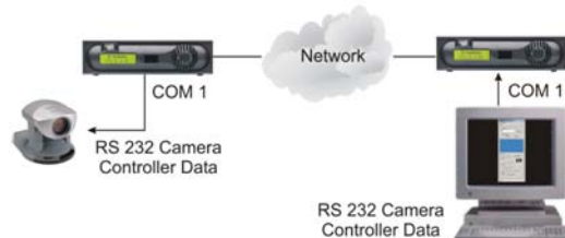
Figure 3. Typical Serial Port Passthrough Configuration
